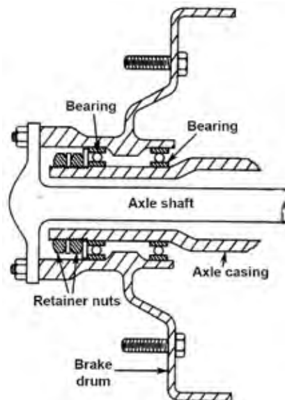
Fig. 4.21 Fully-floating Rear Axle
