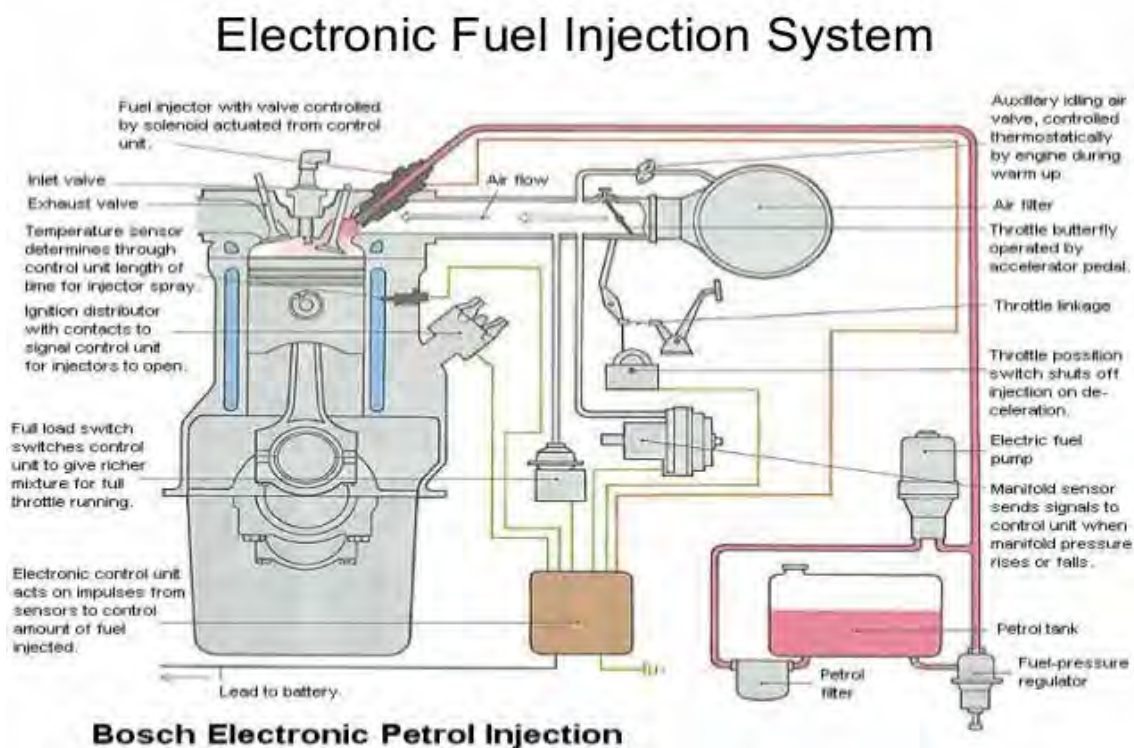
Fig. 5.29: Electronic Fuel Injection System
