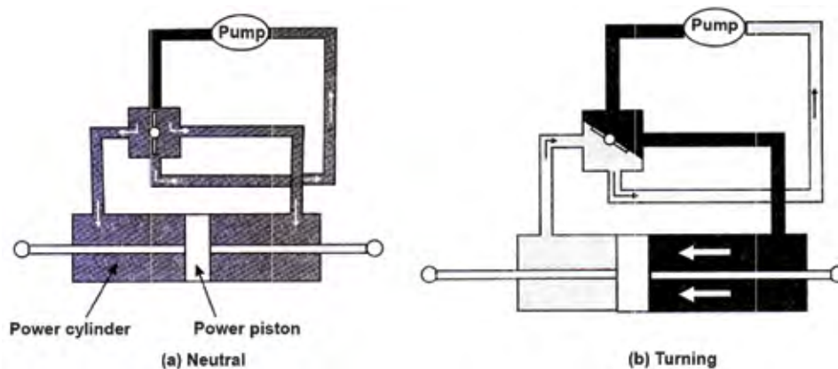
Fig. 2.16 Working Principle of Hydraulic Power Steering.
