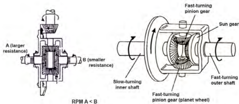
Fig. 4.17 Operation of Differential while vehicle taking a turn
