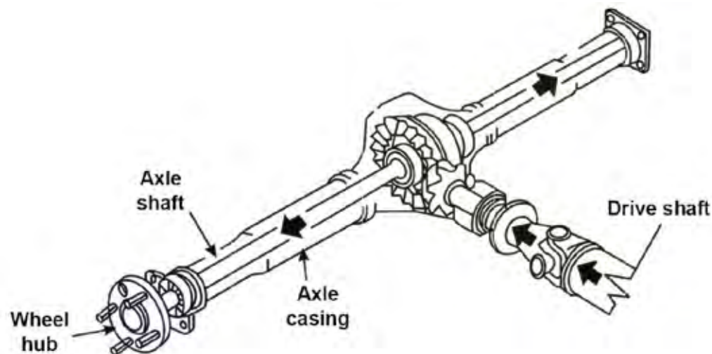
Fig. 4.18 Rear Axle Assembly
