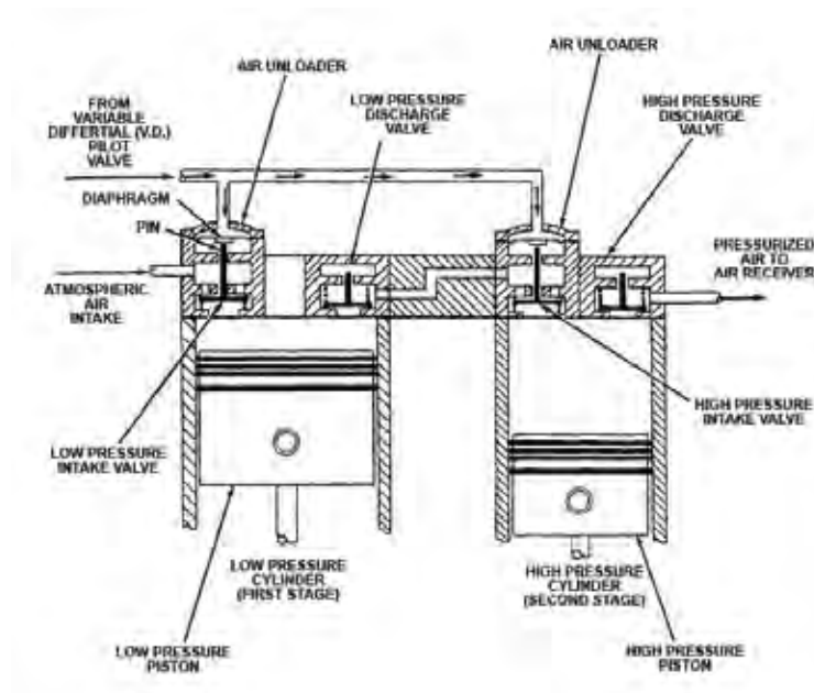
Fig. 1.1 Air Compressor
