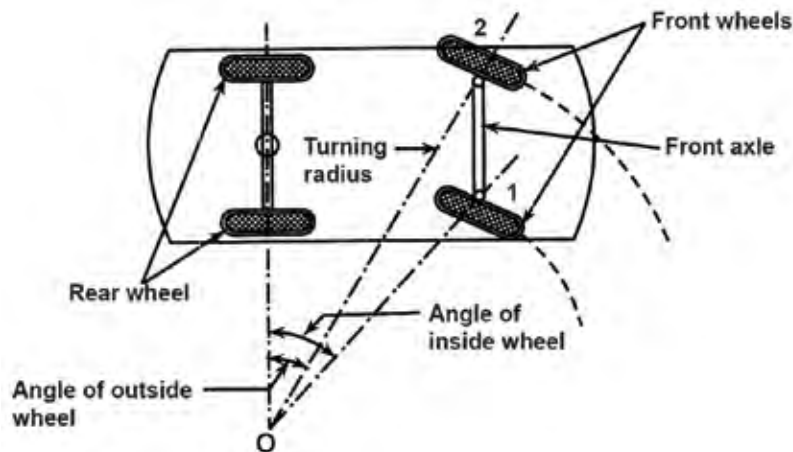
Fig. 2.8 Turning Radius
