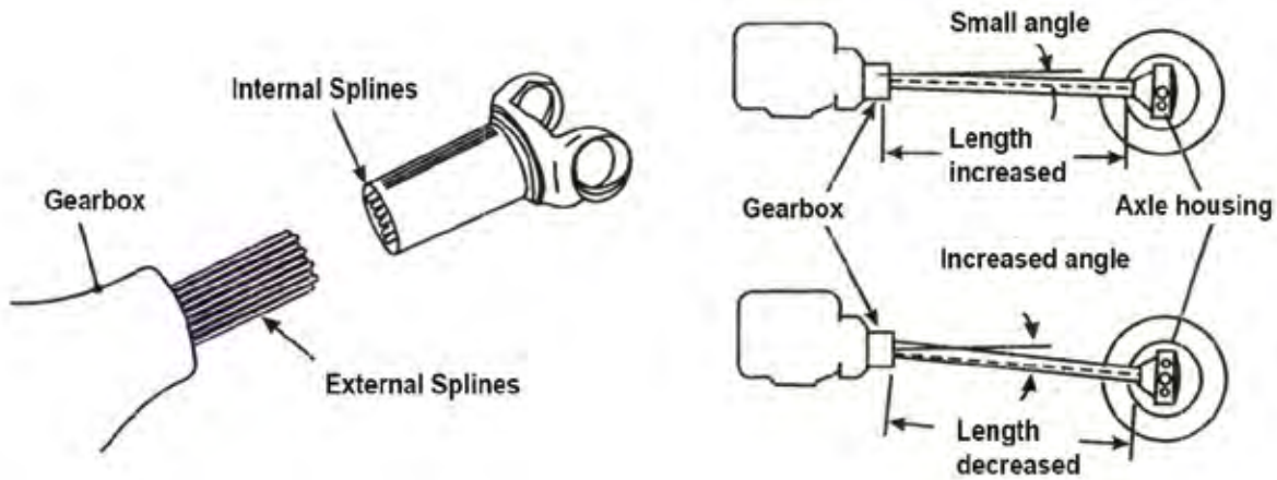
Fig. 4.4 Slip joint and its function
