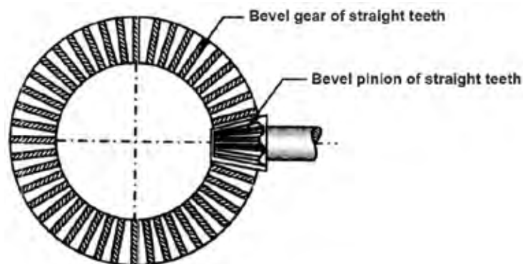
Fig. 4.11 Straight bevel gear drive
