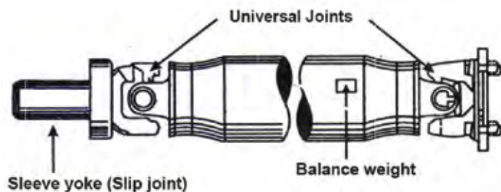
Fig. 4.1 Propeller Shaft Assembly
