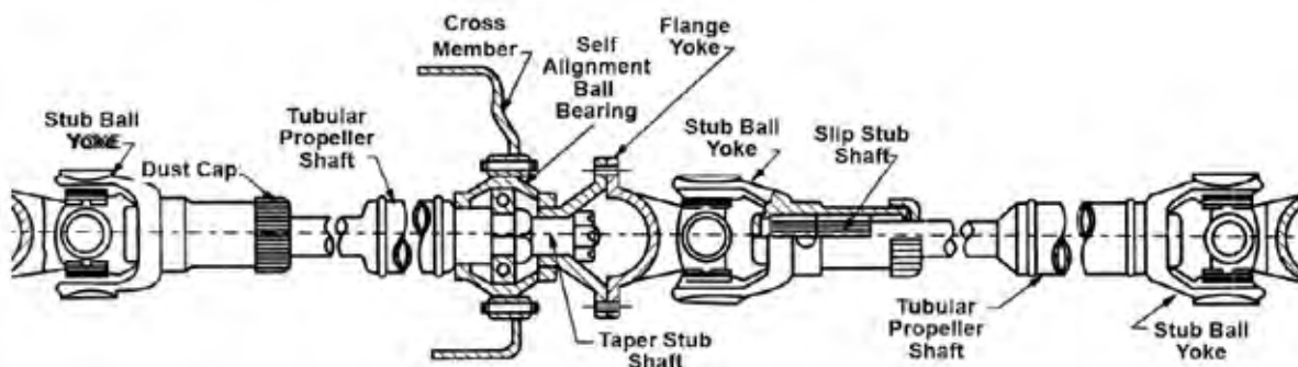
Fig. 4.5 Two-piece Propeller shaft with self alignment Centre Bearing.
