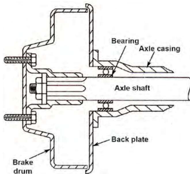
Fig. 4.19 Semi-floating Rear Axle
