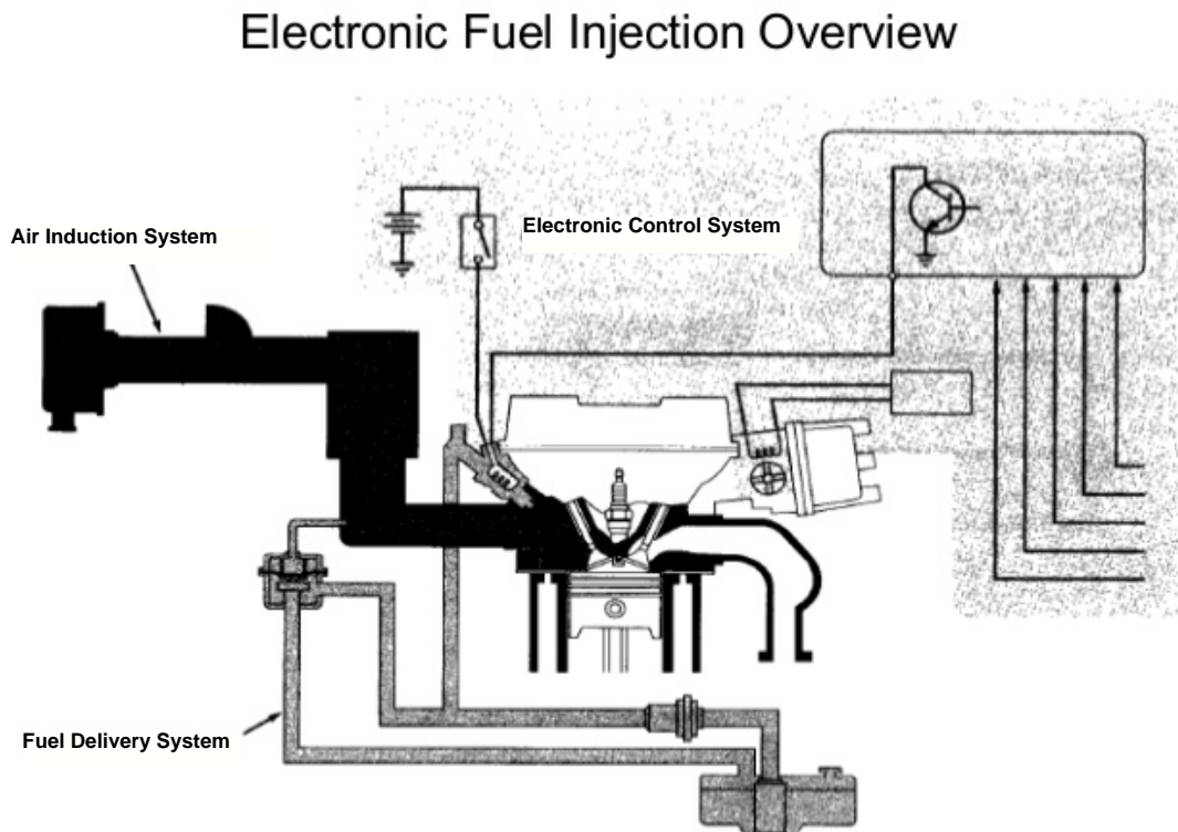
Fig. 5.30: Electronic Fuel Injection overview
