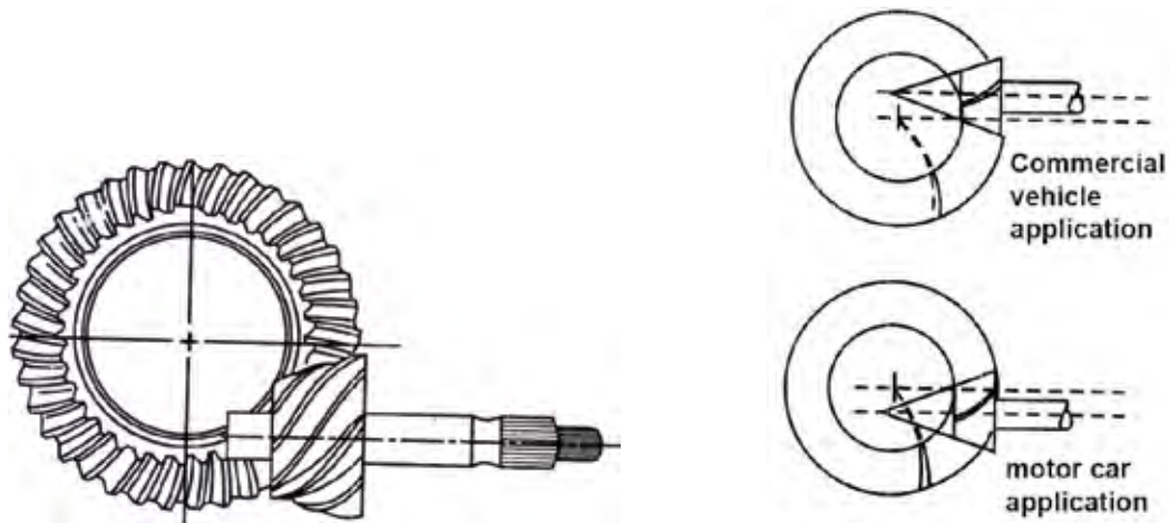
Fig. 4.13 Hypoid gear drive
