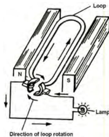
Fig. 5.4 Simple Generator
