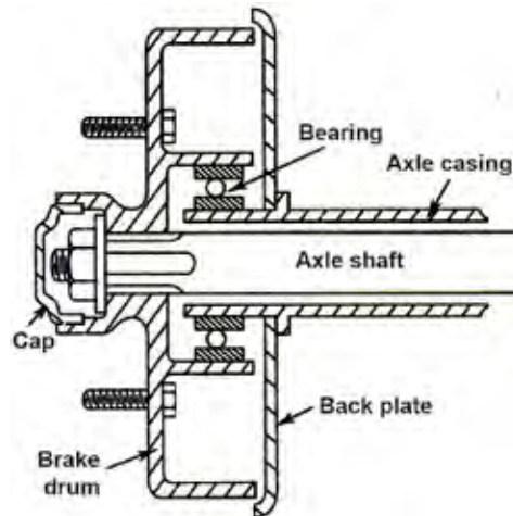
Fig. 4.20 Three-quarter floating Rear Axle
