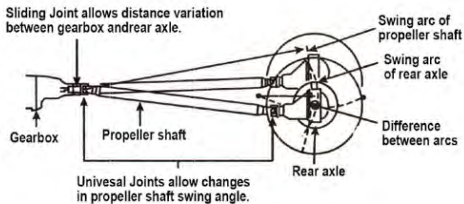
Fig. 4.3 Components and Swing Arc of Propeller shaft and Rear Axle.
