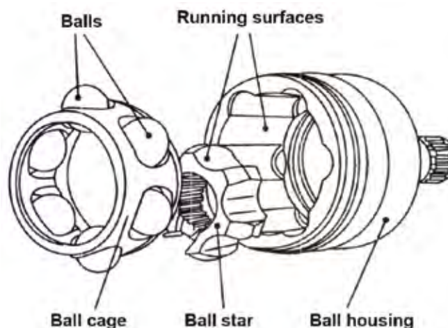
Fig. 4.9 Rzeppa Joint
