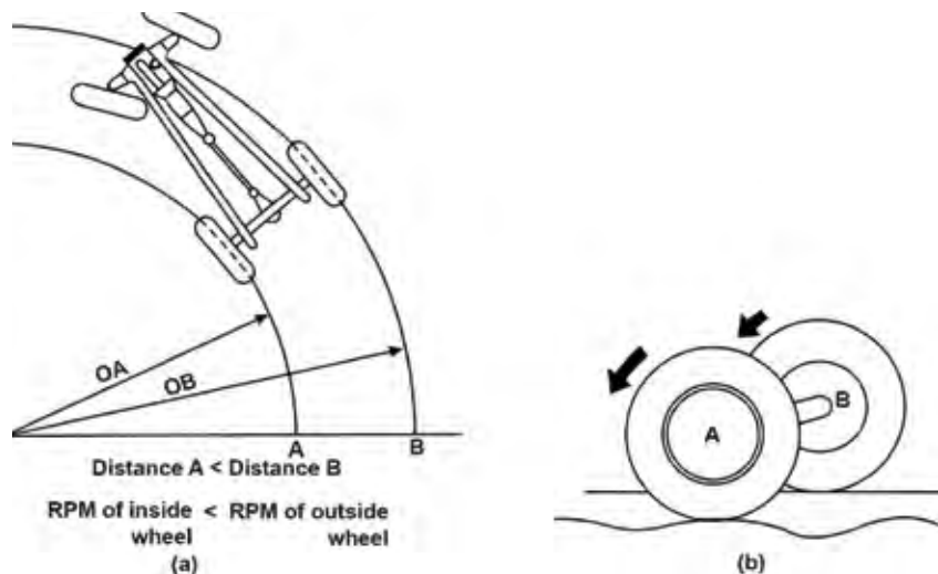
Fig. 4.14 Principle of Differential
