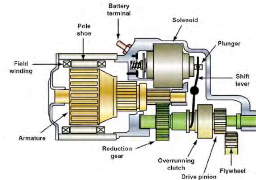
Fig. 5.24 Drive Mechanism of Starter Motor.
