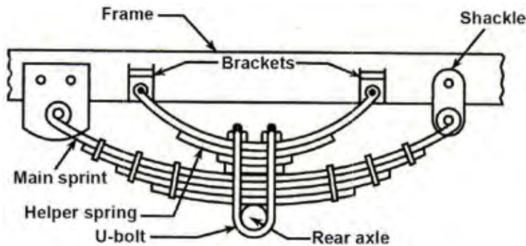
Fig. 3.9 Helper Springs
