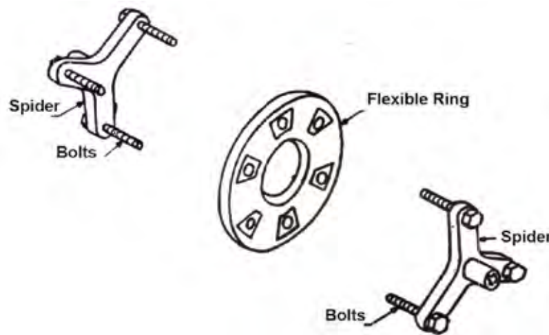
Fig. 4.7 Flexible Ring type Universal Joint
