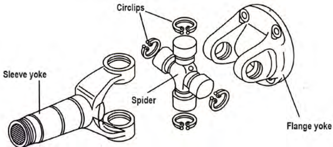
Fig. 4.6 Cross or Spider type Universal Joint
