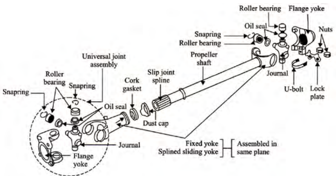
Fig. 4.2 Exploded view of various components of Propeller shaft and Universal Joint.
