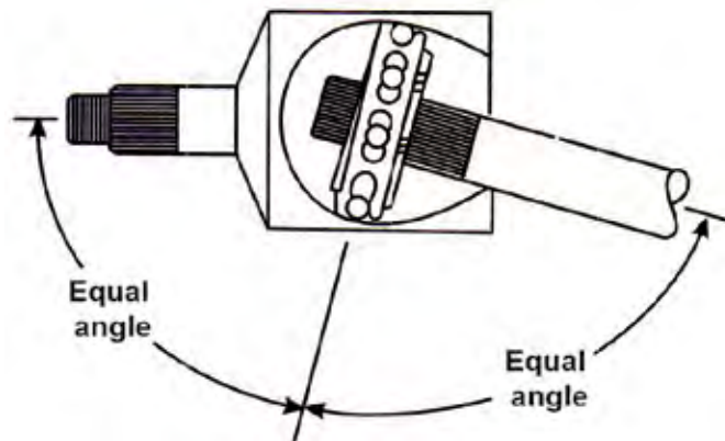
Fig. 4.8 Constant Velocity Joint
