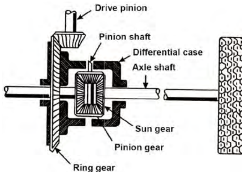
Fig. 4.15 Differential Assembly
