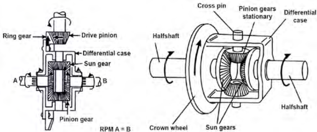
Fig. 4.16 Operation of Differential while vehicle moving on straightahead
