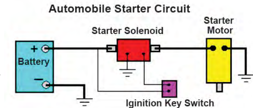
Fig. 5.17 Starting Circuit
