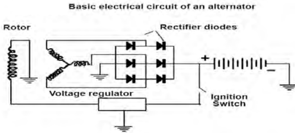
Fig. 5.16 Basic Electrical Circuit of Alternator.
