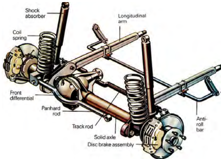
Fig. 3.1 Rigid Axle Suspension System with coil springs and shock absorber
