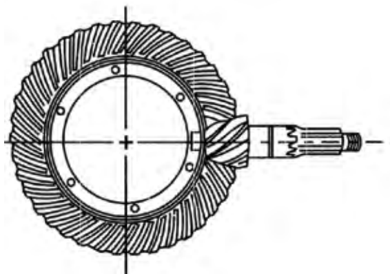
Fig. 4.12 Spiral bevel gear drive
