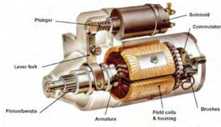
Fig. 5.23 Starter Motor Assembly Complete.
