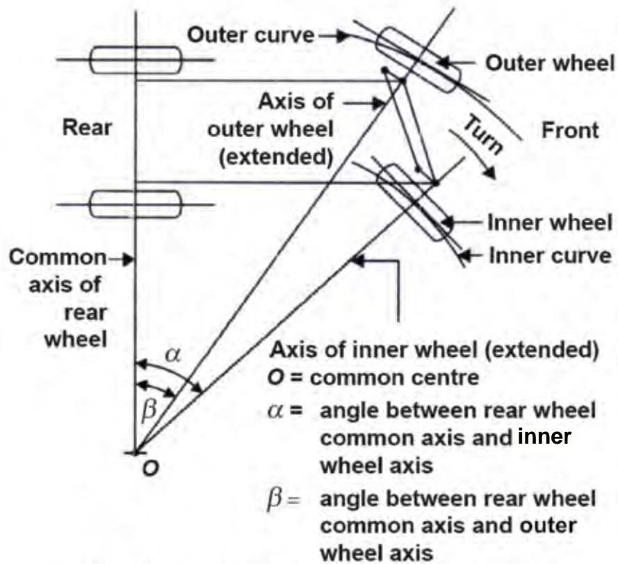
(b) Ackerman's steering principle (right turn)
