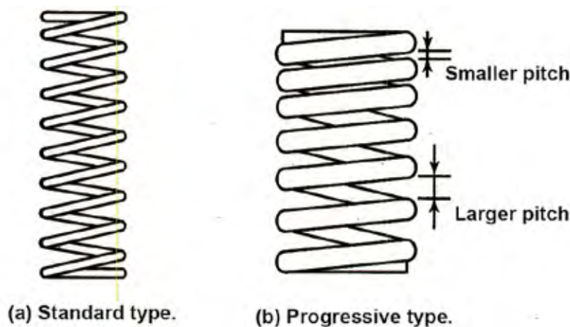
Fig. 3.13 Coil Spring
