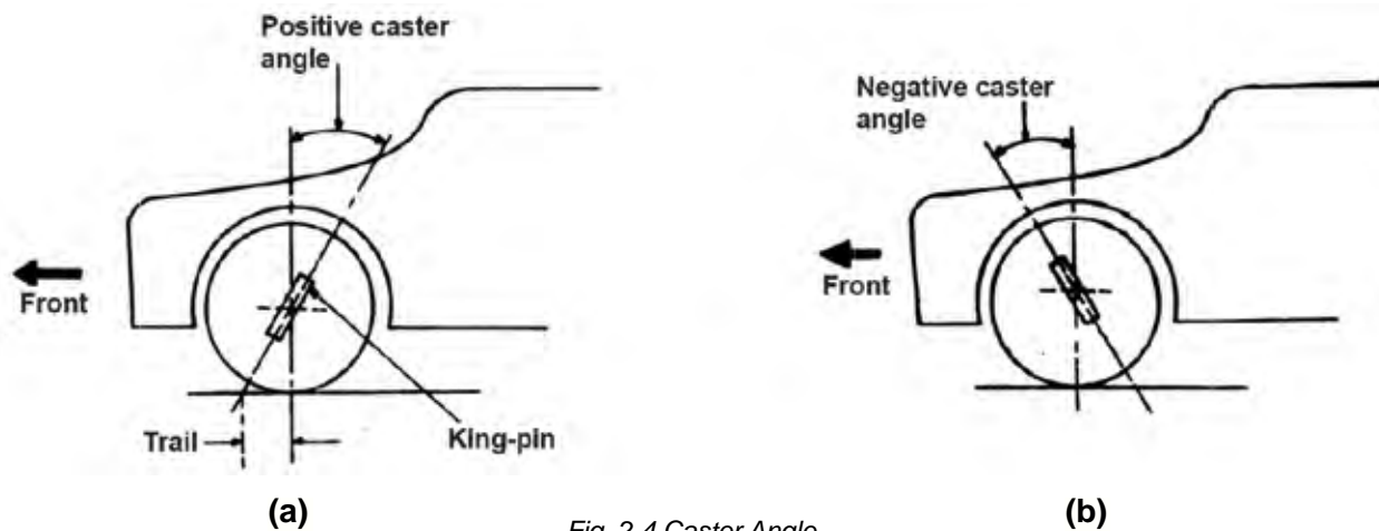
Fig. 2.4 Caster Angle
