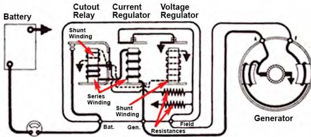
Fig. 5.11 Three unit Regulator.
