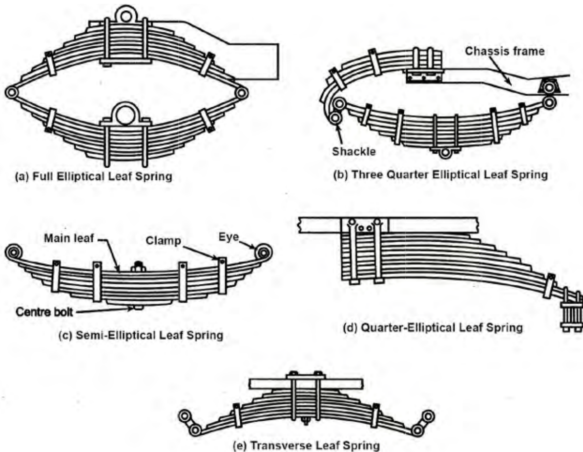
Fig. 3.8 Different types of Leaf Springs
