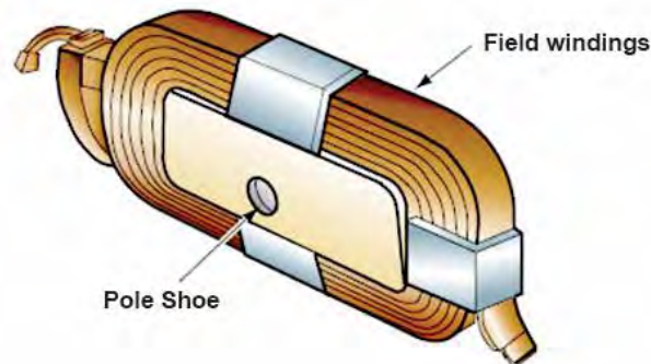
Fig. 5.22 Pole Shoe & Field Winding of Starter Motor.
